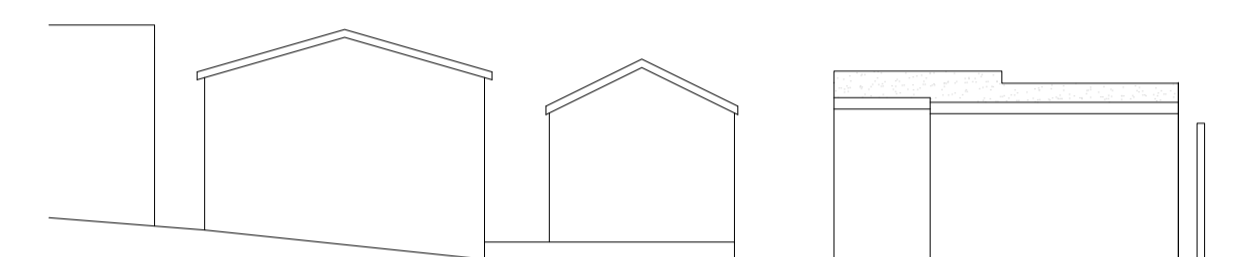
Proposed Structures West Facing Elevation 1:100
